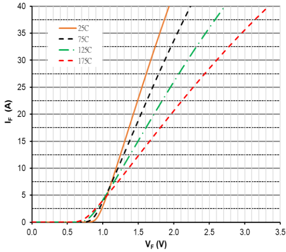
Figure 1. Forward Characteristics
