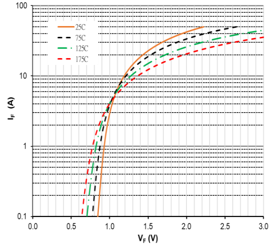
Figure 2. Forward Characteristics
